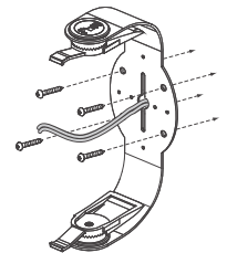
FIGURE 4: ATTACH BRACKET
