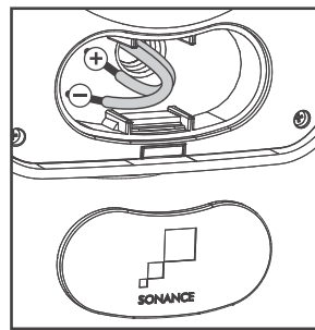
FIGURE 9: CONNECTION TERMINALS
