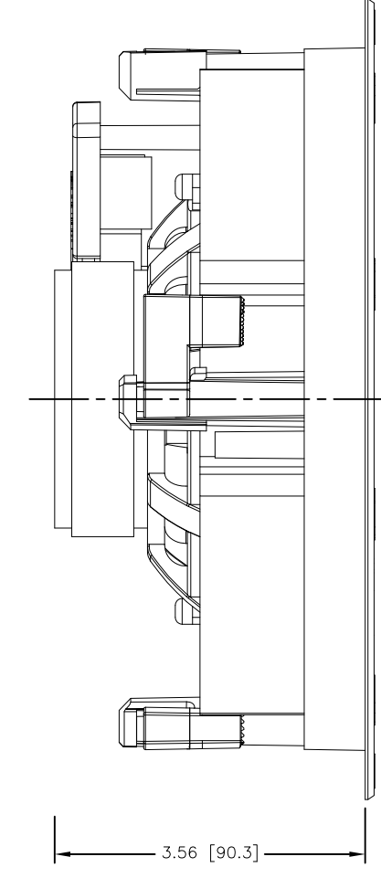
MOUNTING DEPTH
