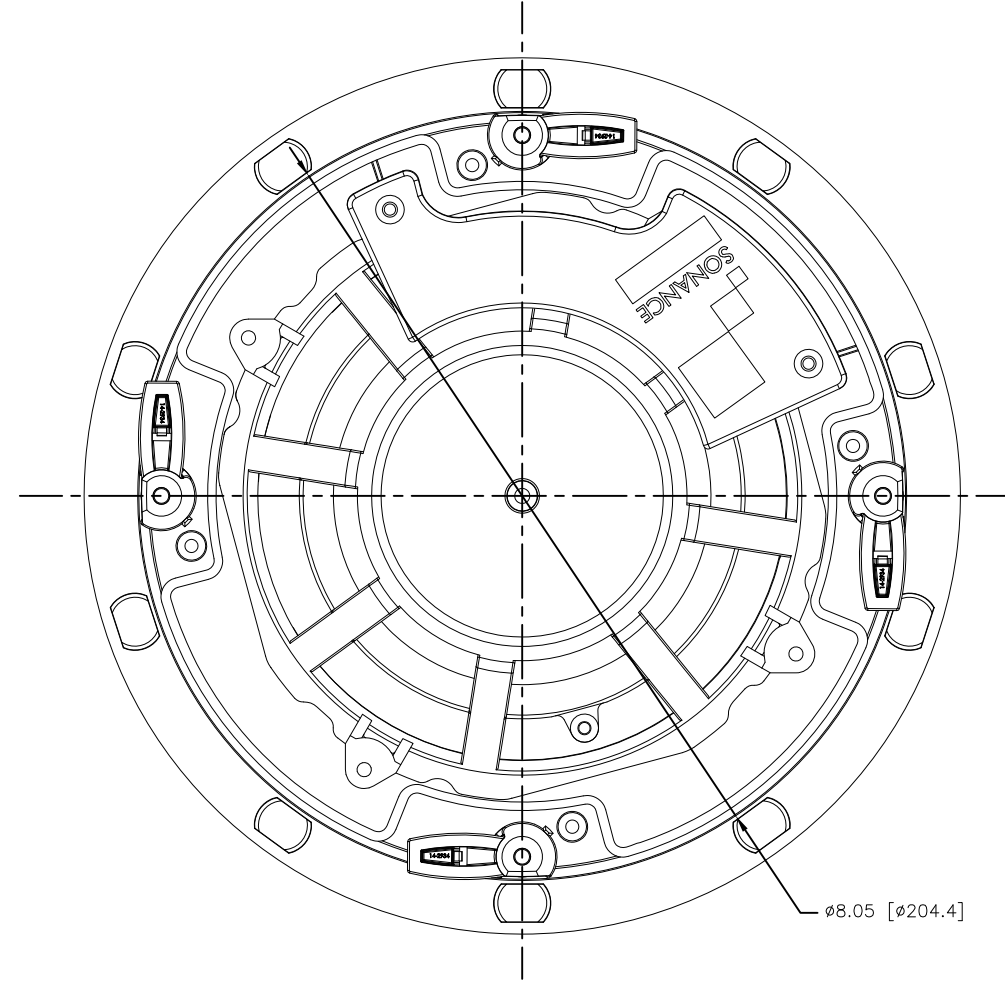
BACK/MINIMUM CUTOUT
