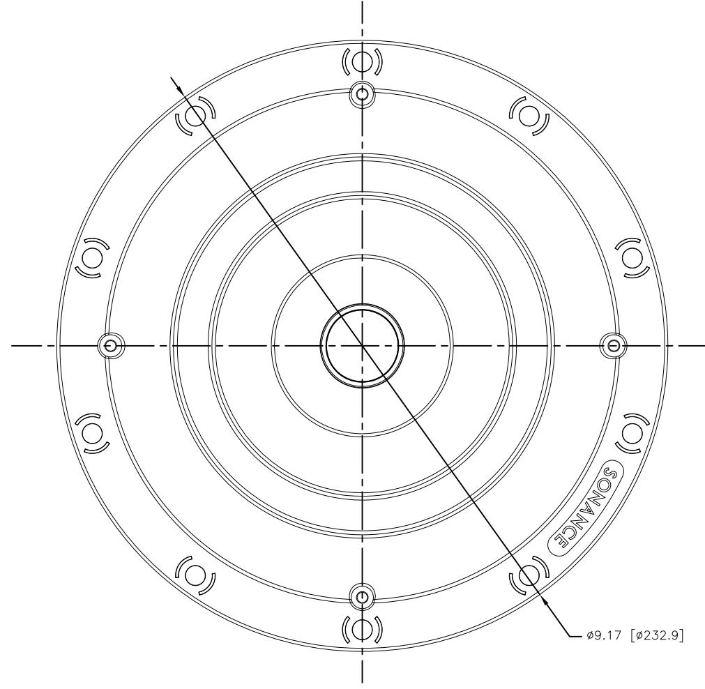
FRONT
