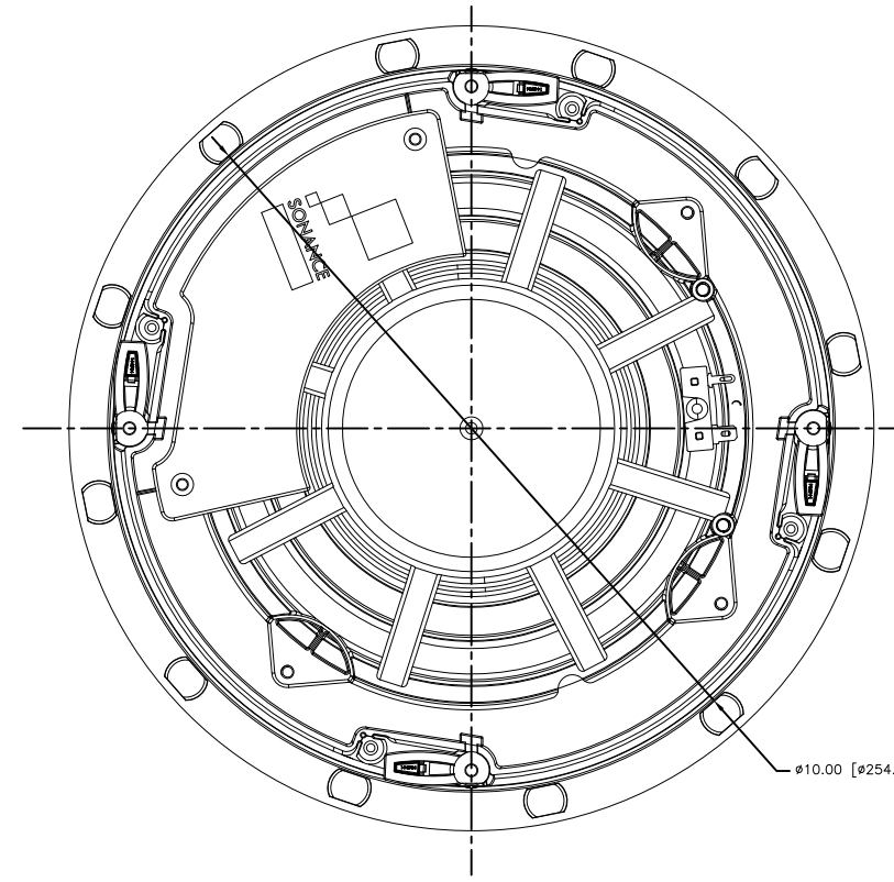
BACK/MINIMUM CUTOUT
